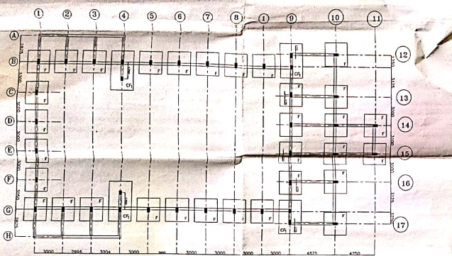
CENTER LINE AND FOUNDATION LAYOUT PLAN WITH BEAM
