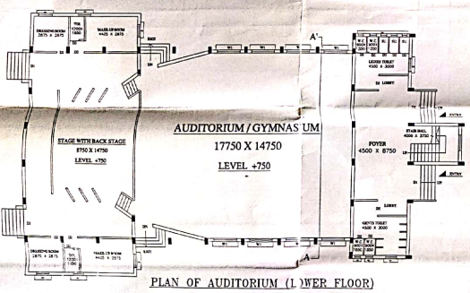
PLAN OF AUDITORIUM (LOWER FLOOR)
